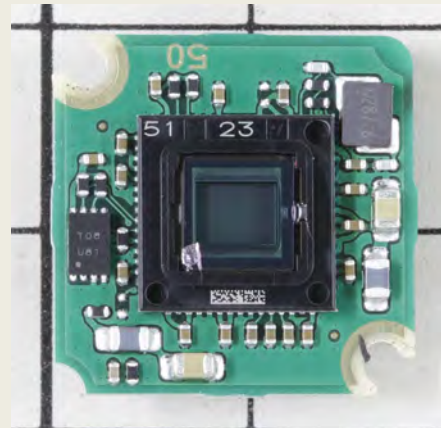
Control unit PCB
